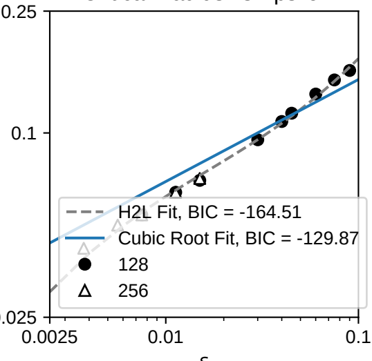
Different Fits of Critical Radius vs Epsilon
